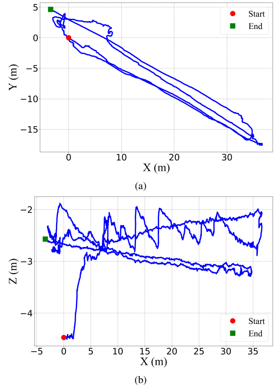
Fig. 3. EKF Odometry based om AHRS, DVL and the pressure sensor. The ROV was deployed and recovered from the same ice hole. a) Top view, (b) X-Z plane. The X-Y plane error distance in the odometry between the start and the end points is 5.75 m.
